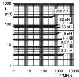
Inductance dependent on frequency
