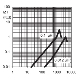
Impedance dependent on frequency
