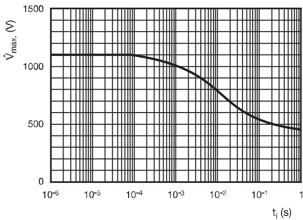
AC01 and AC01-AT Pulse on a regular basis; max. permissible peak pulse voltage ( \hat{V}_{max} ) as a function of pulse duration ( t_i )
