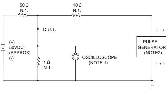
FIG.1 – REVERSE RECOVERY TIME AND CHARACTERISTIC TEST CIRCUIT DIAGRAM
