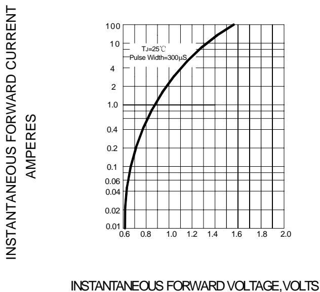
FIG.4–TYPICAL FORWARD CHARACTERISTIC
