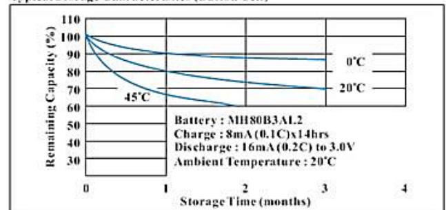
Typical Storage Characteristics (Button Cell)
