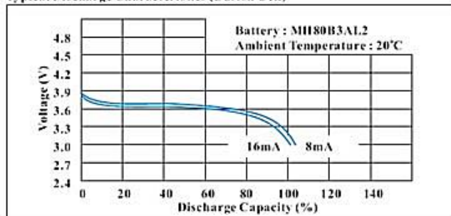
Typical Discharge Characteristics (Button Cell)
