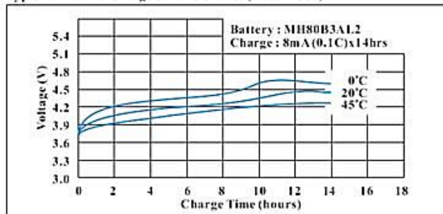
Typical Quick Charge Characteristics (Button Cell)
