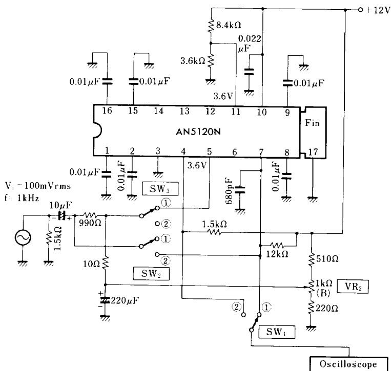
Test Circuit 3 ( G_{V(1)} , G_{V(2)} )
