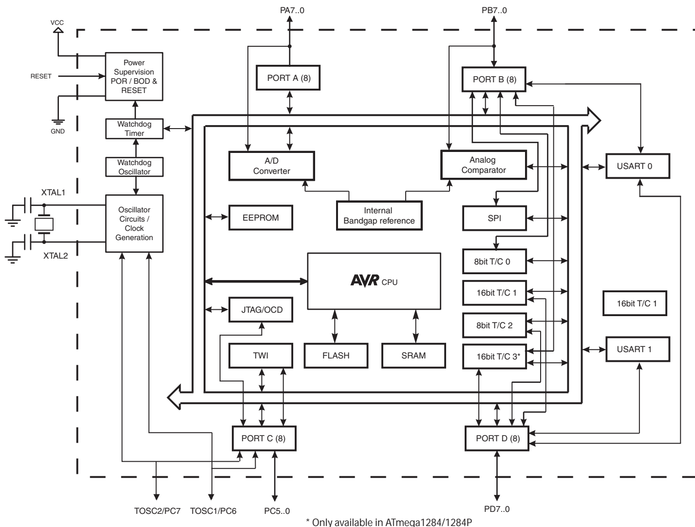
Figure 2-1. Block diagram.
