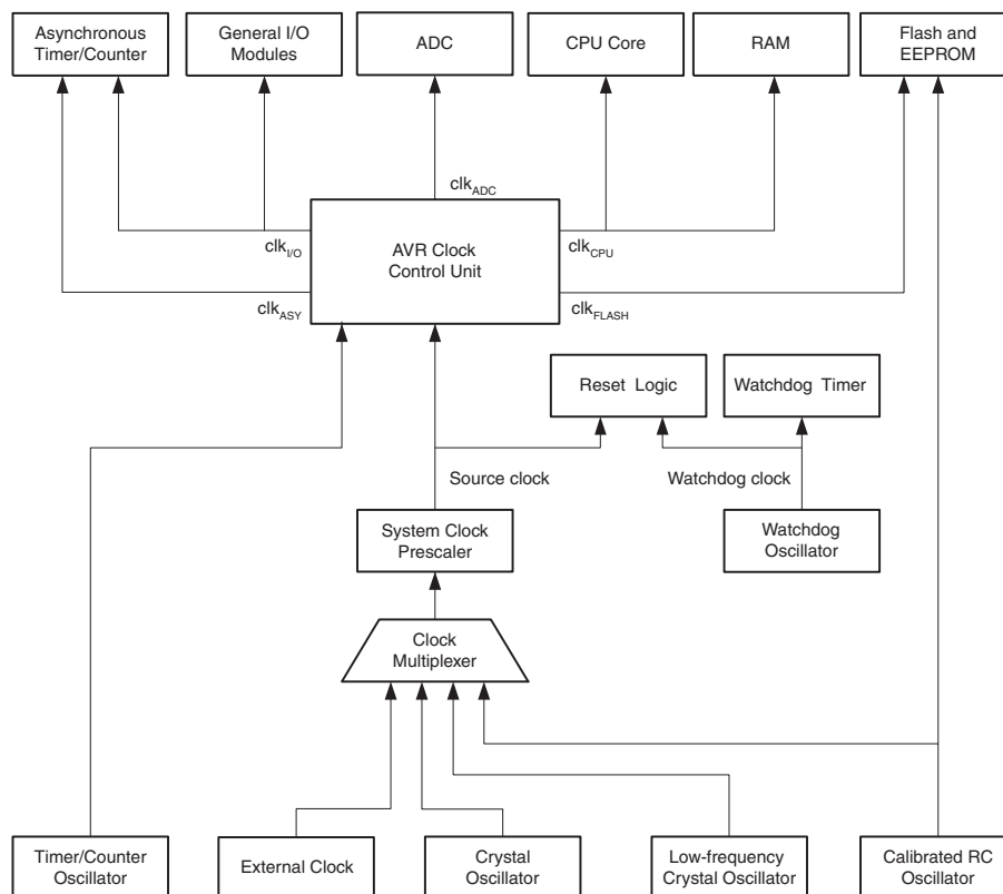
Figure 9-1. Clock distribution.
