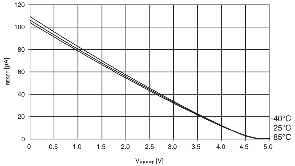
Figure 29-364. Atmel ATmega1284P: Reset pull-up resistor current vs. reset pin voltage ( V_{CC} = 5V ).
