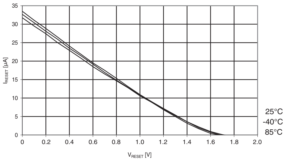
Figure 29-214. Atmel ATmega644A: Reset pull-up resistor current vs. reset pin voltage ( V_{CC} = 1.8V ).
