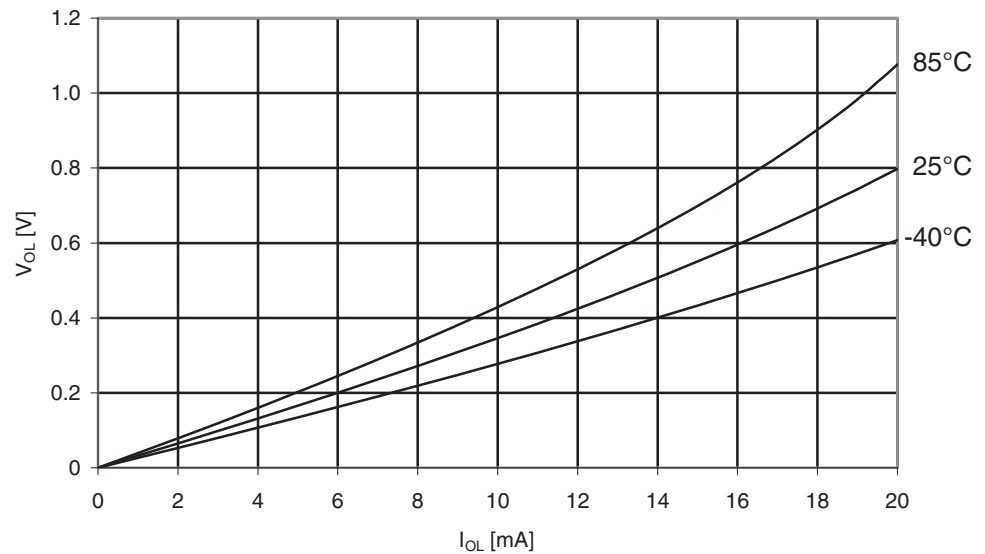
Figure 29-315. Atmel ATmega1284: I/O pin output voltage vs. sink current ( V_{CC} = 2.7V ).
