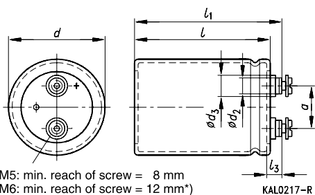
Type B43560 Ring clip/clamp mounting
