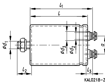
Type B43580 Threaded stud mounting
