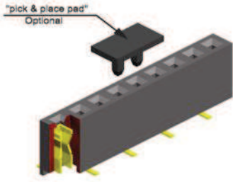
Foot style
