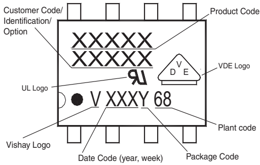
Figure 14. Marking example
