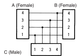
Internal Connections
