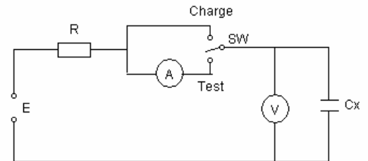
Measurement circuit
