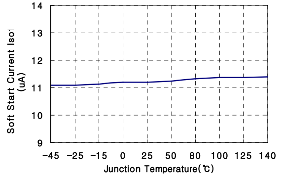
Figure 15. Soft-Start Current
