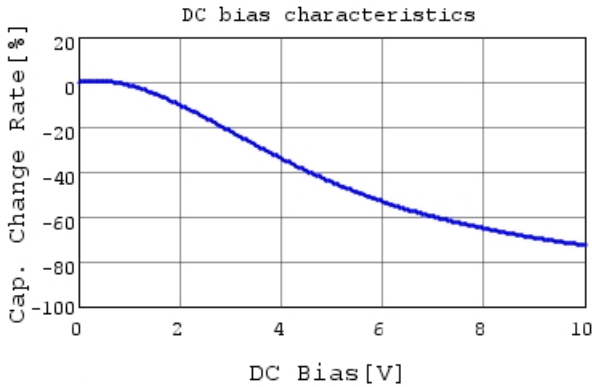
GCM155C71A105KE38 C-DC bias capchange, 25.0c
