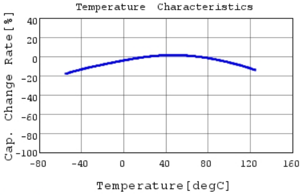
GCM155C71A105KE38 C-Temp. capchange, DC0.0V,
