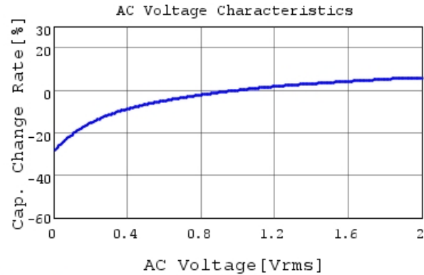
GCM155C71A105KE38 C-AC Voltage capchange, Dc
