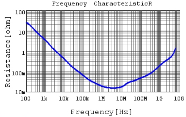
GCM155C71A105KE38 R DCOV, 25degC
