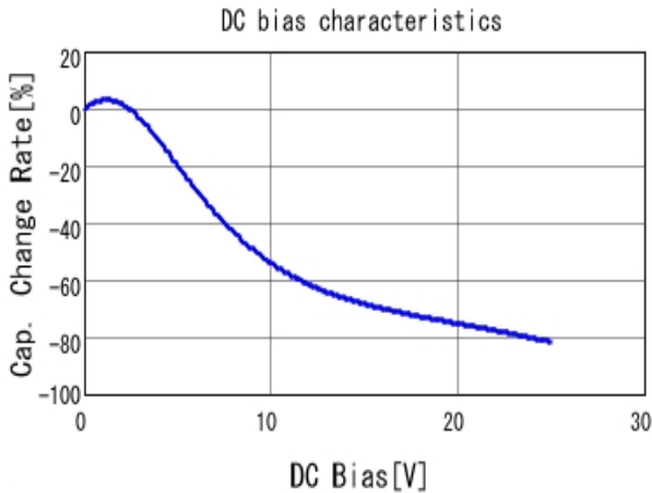
■ GRM32ER71E226ME15 C-DC bias capchange, 25.0degC, AC0.
