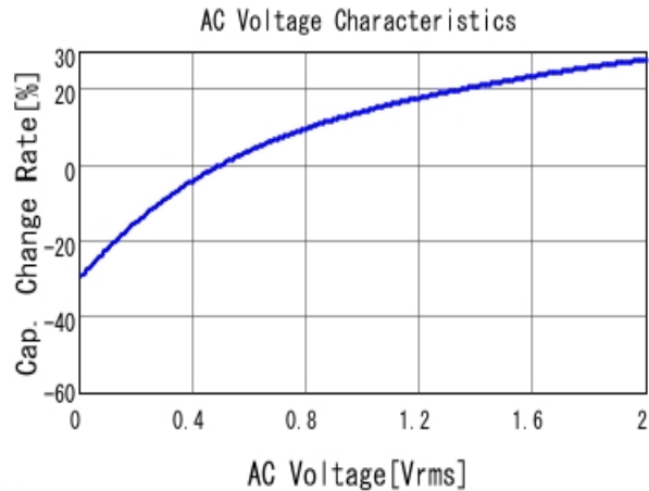
■ GRM32ER71E226ME15 C-AC Voltage capchange, DCOV, 25.0d
