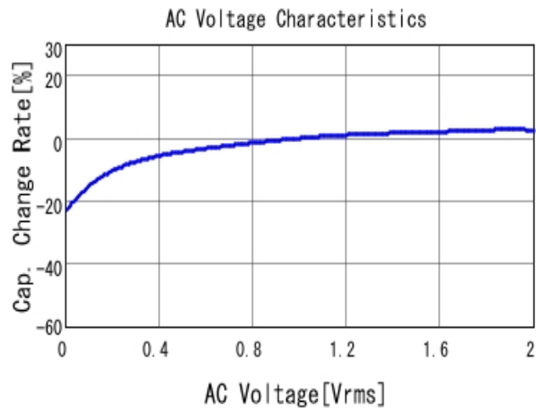
■ GRT155R61E225KE13 C-AC Voltage capchange, DCOV, 25.0d
