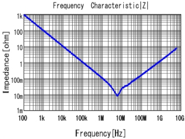
■ GRT155R61E225KE13 |Z| DCOV, 25degC
