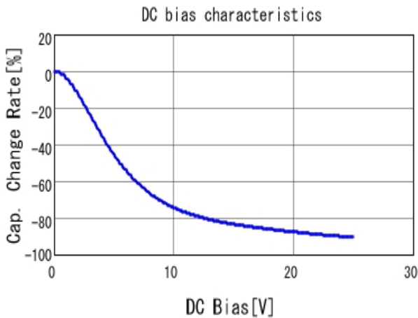
■ GRT155R61E225KE13 C-DC bias capchange, 25.0degC, AC1V
