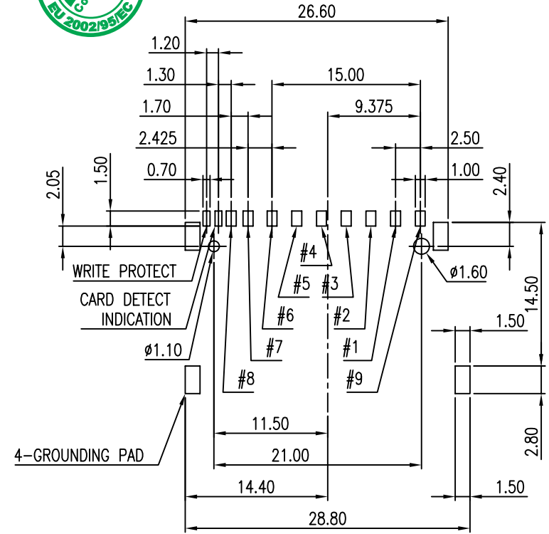
RECOMMENDED PCB LAYOUT (ALL TOLERANCES ARE ±0.05)
