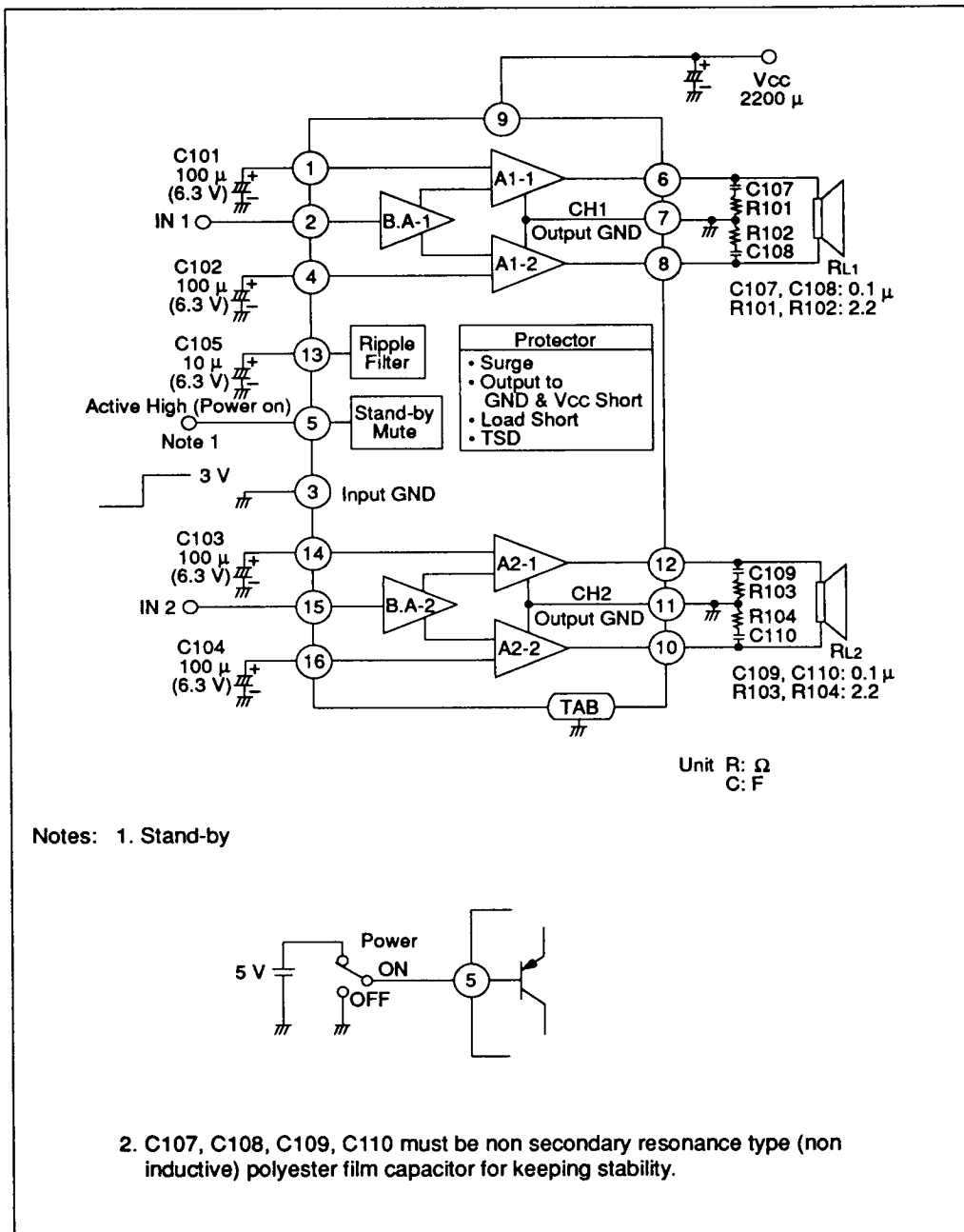
Figure 1 Block Diagram
