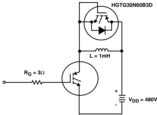
FIGURE 19. INDUCTIVE SWITCHING TEST CIRCUIT
