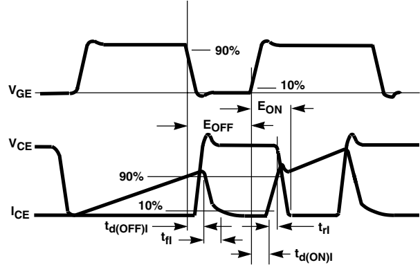
FIGURE 20. SWITCHING TEST WAVEFORMS
