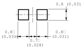
Figure 10. Recommended Soldering Pattern for HSMB-C190 and C191.
