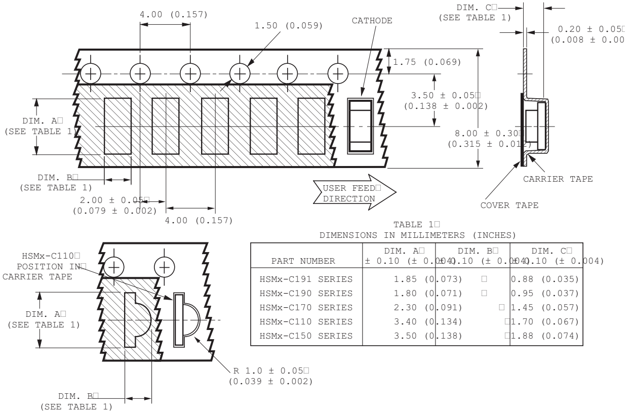
Figure 15. Tape Dimensions.
