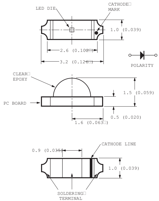
HSMx-C110
