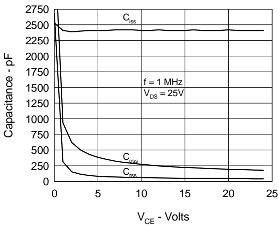
Fig.9 Capacitance Curves
