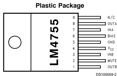
Package Description Top View Order Number LM4755T Package Number TA09A
