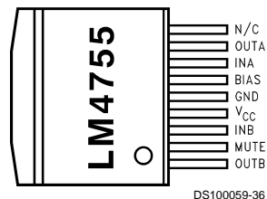
Top View Order Number LM4755TS Package Number TS9A
