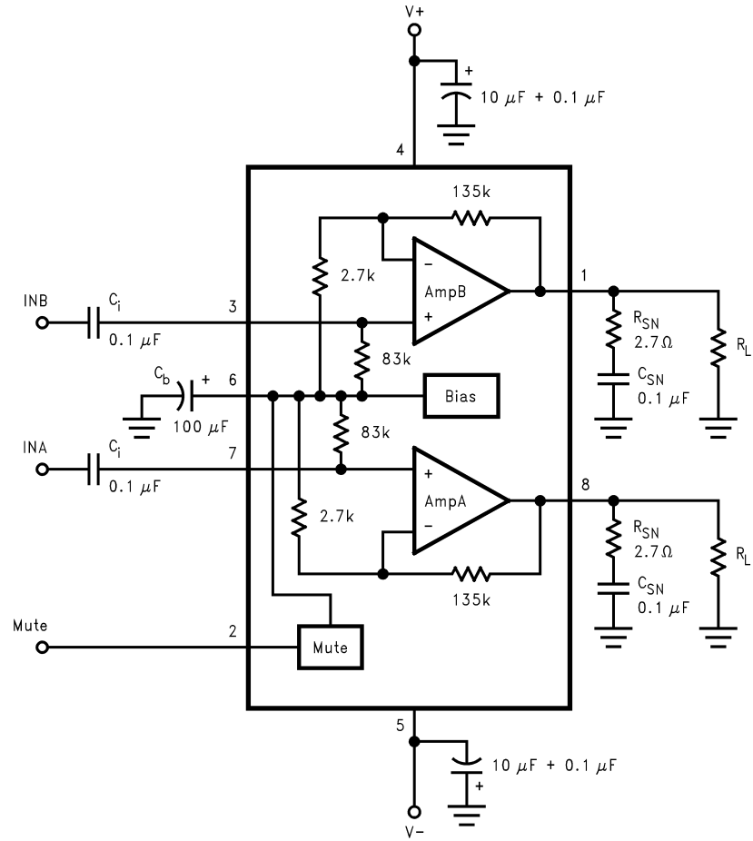
FIGURE 2. Test Circuit
