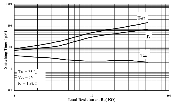
Figure 16. Switching Time vs. Load Resistance
