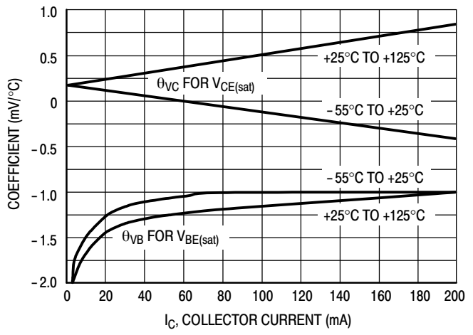
Figure 20. Temperature Coefficients
