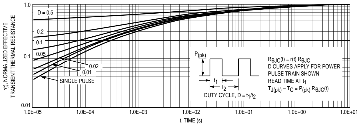
Figure 13. Thermal Response
