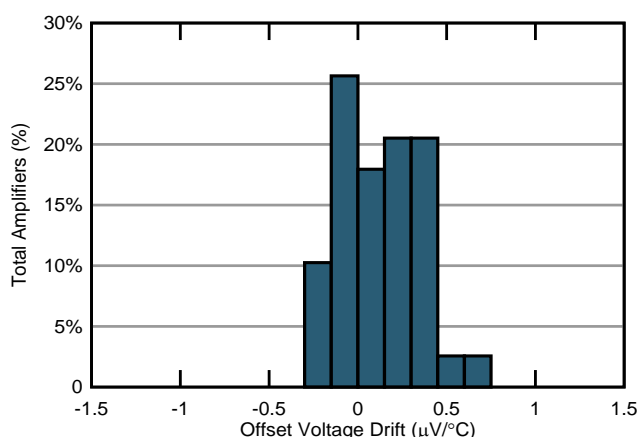
Offset Voltage Drift
