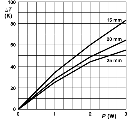
\varnothing 0.78 mm Cu-leads Minimum distance from resistor body to PCB = 1 mm PR03 Temperature rise ( \Delta T ) at the lead end (soldering point) as a function of dissipated power at various lead lengths after mounting.
