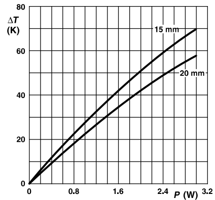
\varnothing 0.78 mm FeCu-leads Minimum distance from resistor body to PCB = 1 mm PR03 Temperature rise ( \Delta T ) at the lead end (soldering point) as a function of dissipated power at various lead lengths after mounting.
