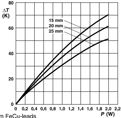
\varnothing 0.78 mm FeCu-leads Minimum distance from resistor body to PCB = 1 mm PR02 Temperature rise ( \Delta T ) at the lead end (soldering point) as a function of dissipated power at various lead lengths after mounting.
