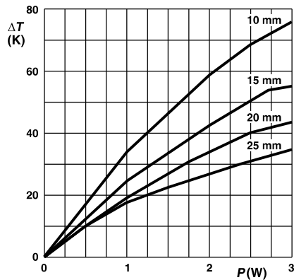
\varnothing 0.58 mm FeCu-leads Minimum distance from resistor body to PCB = 1 mm PR03 Temperature rise ( \Delta T ) at the lead end (soldering point) as a function of dissipated power at various lead lengths after mounting.
