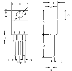
TO-220AB
