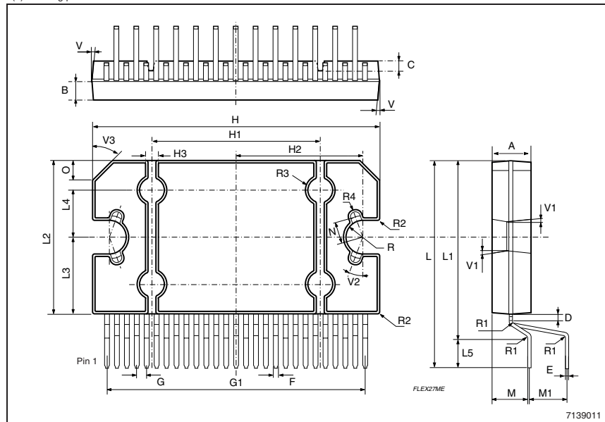
Flexiwatt27 (vertical)
