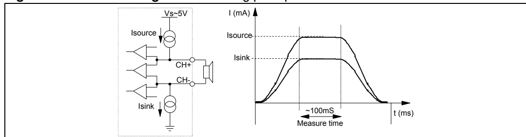
Figure 19. Turn - on diagnostic: working principle
