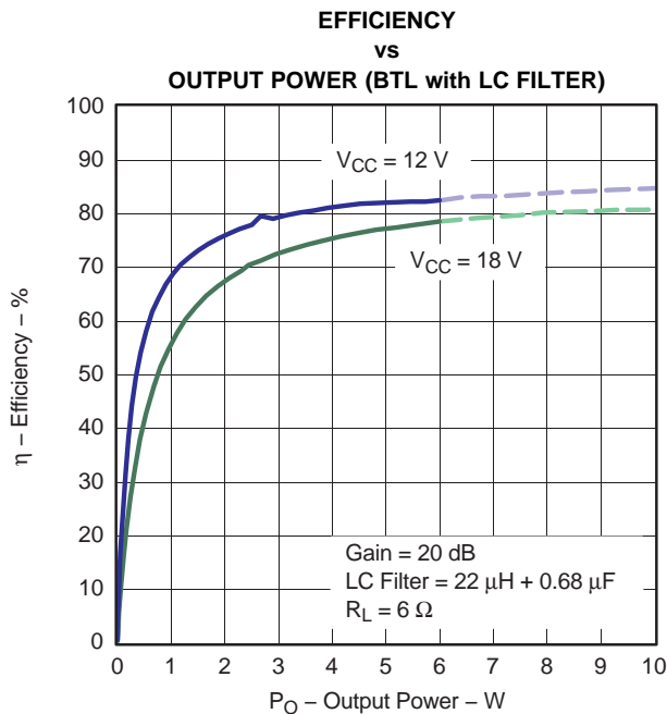
NOTE: Dashed lines represent thermally limited region. Figure 20.
