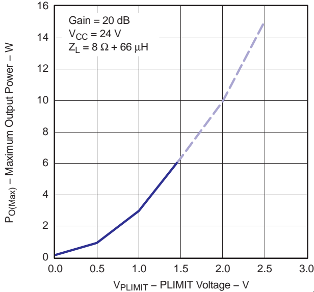
MAXIMUM OUTPUT POWER vs PLIMIT VOLTAGE (BTL)
