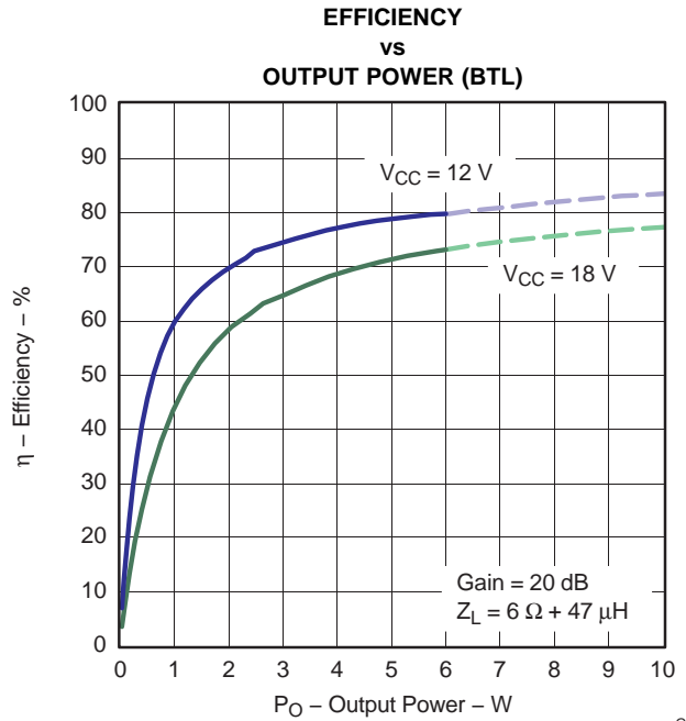
NOTE: Dashed lines represent thermally limited region. Figure 19.
