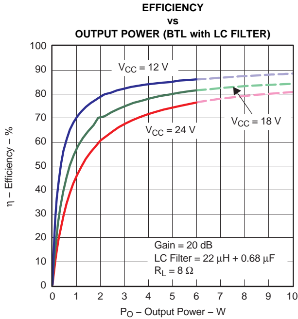
NOTE: Dashed lines represent thermally limited region. Figure 18.
