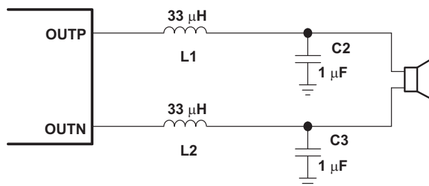
Figure 37. Typical LC Output Filter, Cutoff Frequency of 27 kHz, Speaker Impedance = 8 \Omega
