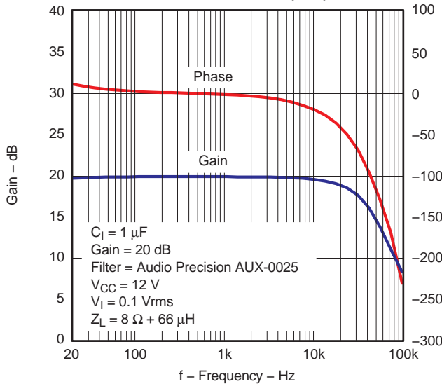
GAIN/PHASE vs FREQUENCY (BTL)
