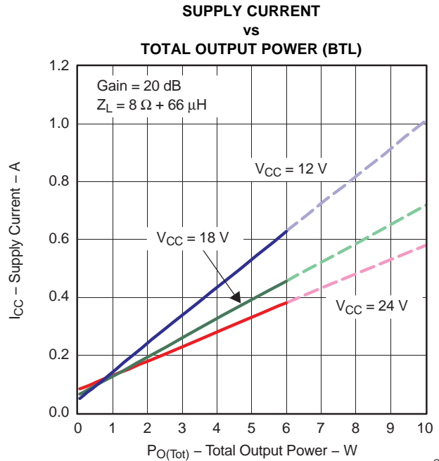
NOTE: Dashed lines represent thermally limited region. Figure 23.
