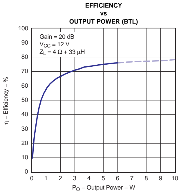
NOTE: Dashed line represents thermally limited region. Figure 21.
