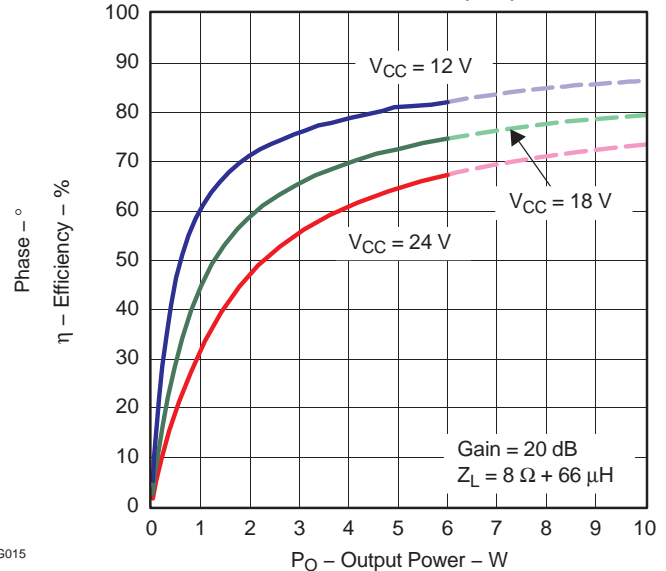
EFFICIENCY vs OUTPUT POWER (BTL)
