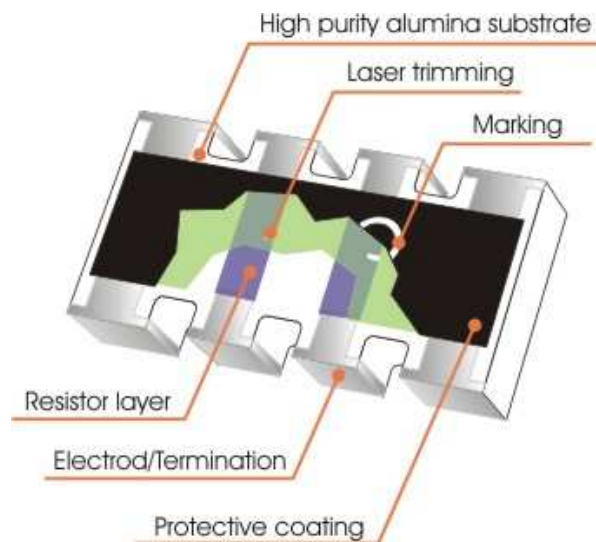
Fig 1. Construction of a Chip-R array WA06X, 5% product
